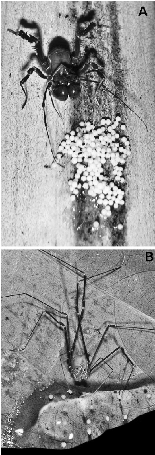
Figure 1.—A. Male of Stenostygnellus aff. flavolimbatus close to a multiple clutch laid on the petiole of a palm. The guarding male is touching the eggs with his second pair of legs (photo: O. Villarreal). B. Female of Eutimesius sp. prostrated close to eggs laid on a leaf and surrounded by an abundant mucus coat (photo: Bejat McCracken).
